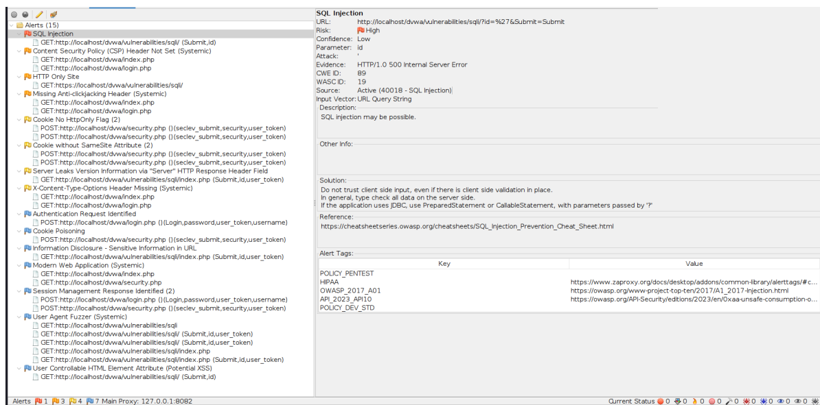
OWASP ZAP's Alerts panel: SQL Injection (CWE-89, High risk) confirmed on the id parameter.
